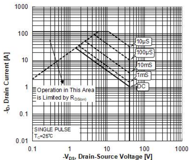
Figure 10a Maximum Safe Operating Area (TO-252)
