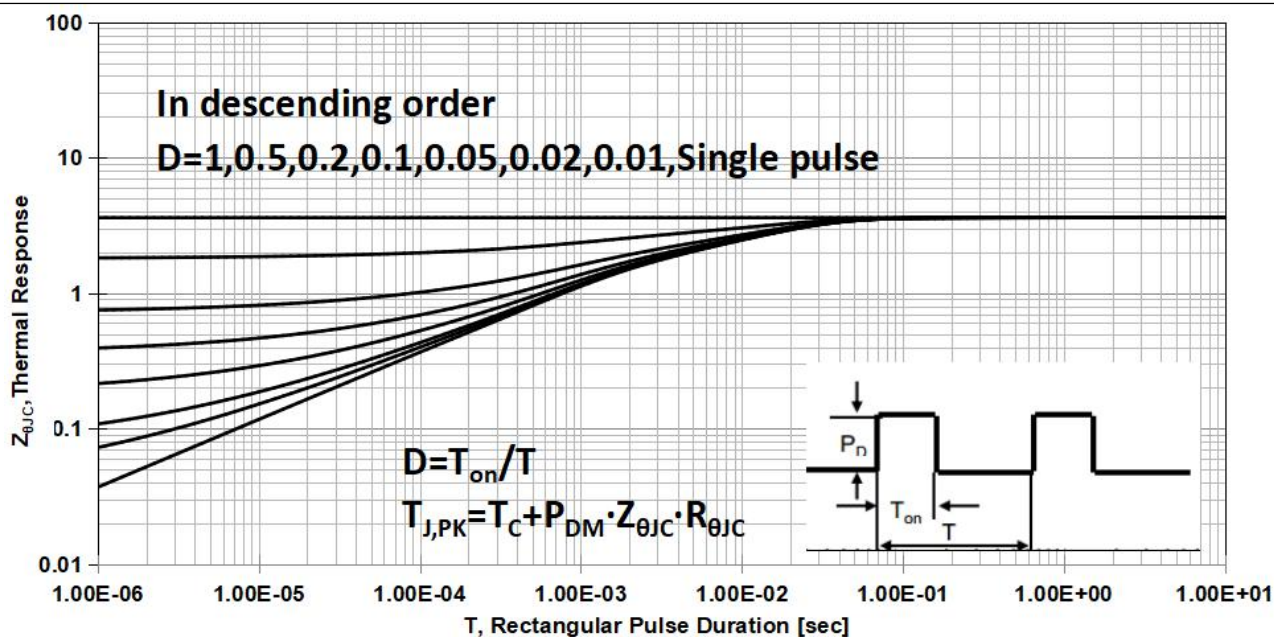
Figure 11a Transient Thermal Impedance(TO-252)
