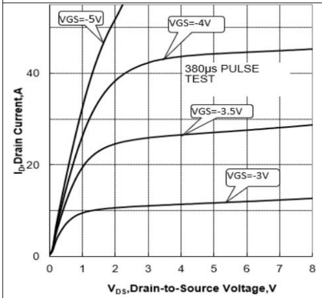
Figure 1 Output Characteristics
