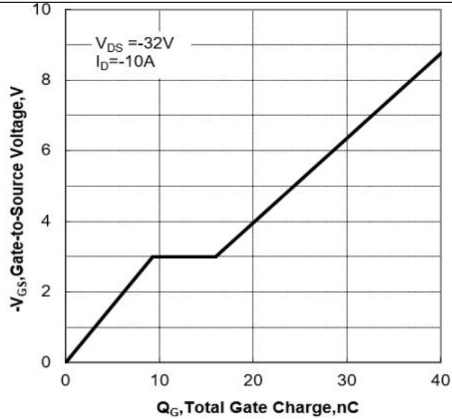
Figure 7 Gate-Charge Characteristics
