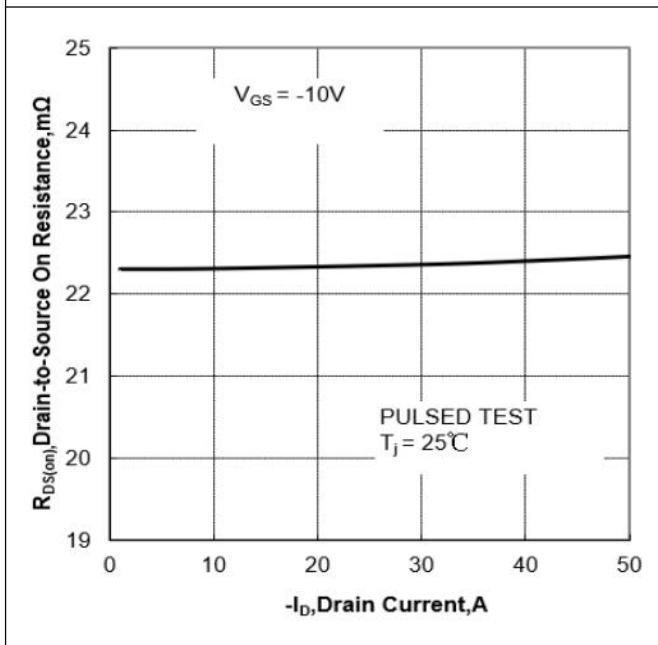
Figure 3 On-Resistance vs. I_D
