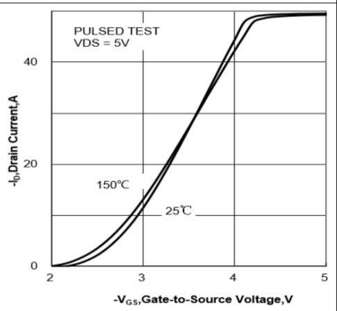
Figure 2 Transfer Characteristics
