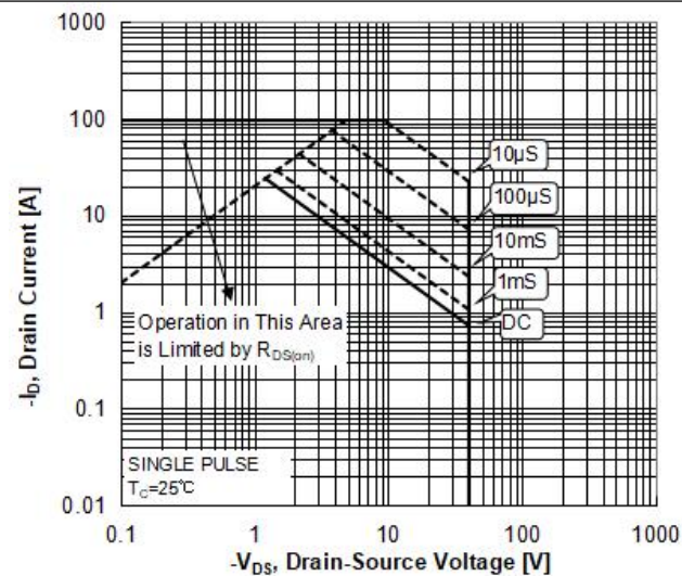
Figure 10c Maximum Safe Operating Area (PDFN3.3*3.3)
