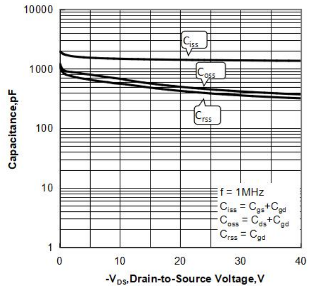
Figure 8 Capacitance Characteristics
