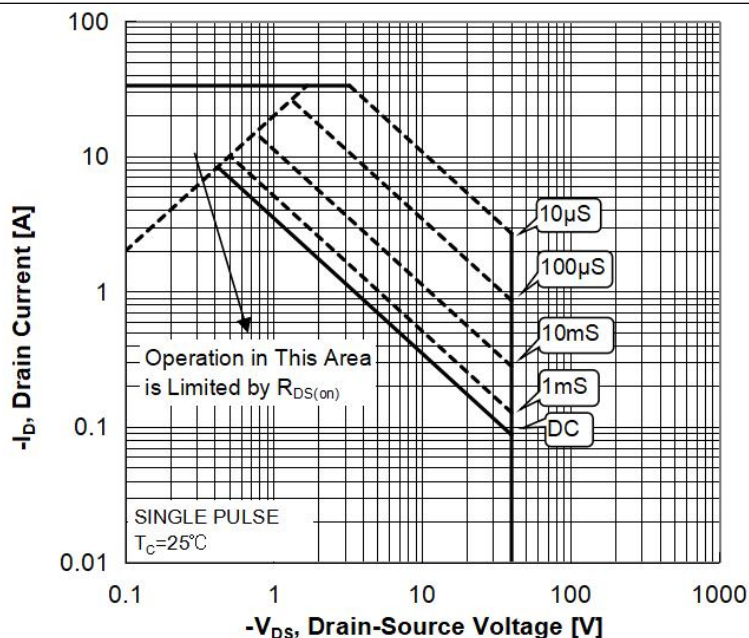
Figure 10d Maximum Safe Operating Area (SOP-8)
