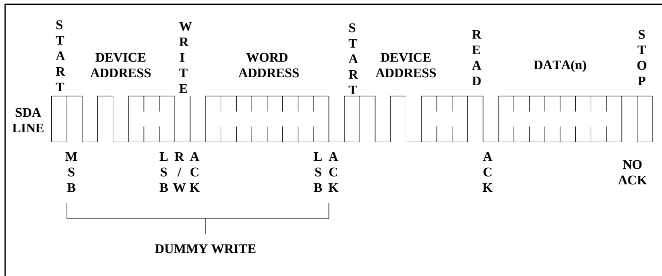
Figure 10. Random Read
