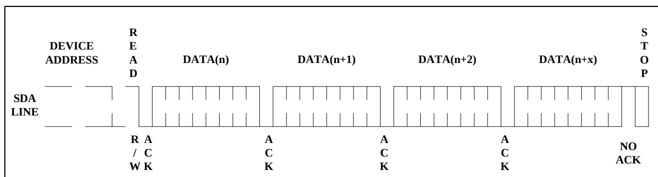
Figure 11. Sequential Read
