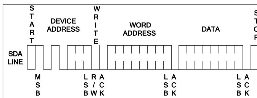
Figure 7. Byte Write
