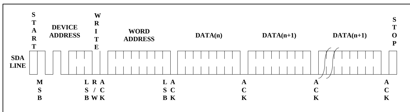
Figure 8. Page Write
