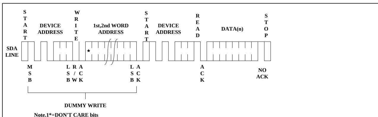
Figure 9. Random Read
