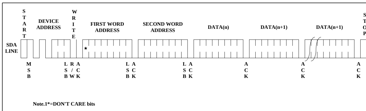
Figure 7. Page Write
