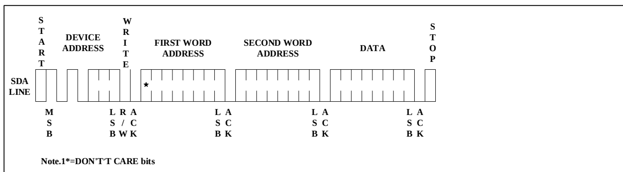
Figure 6. Byte Write
