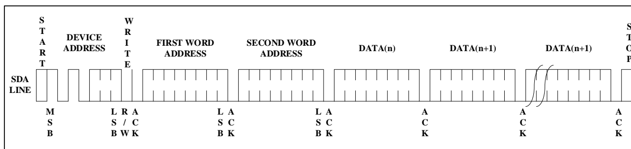
Figure 7. Page Write
