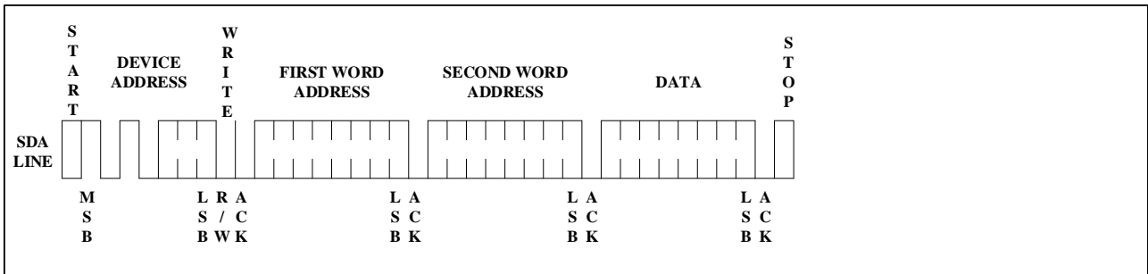
Figure 6. Byte Write
