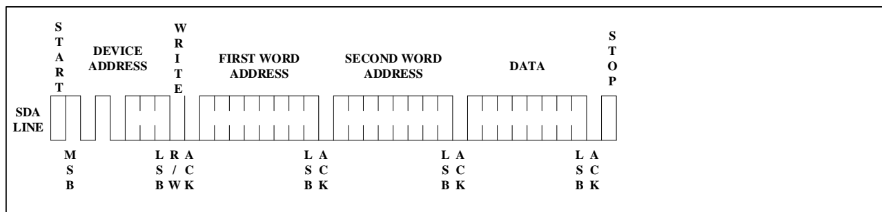
Figure 6. Byte Write
