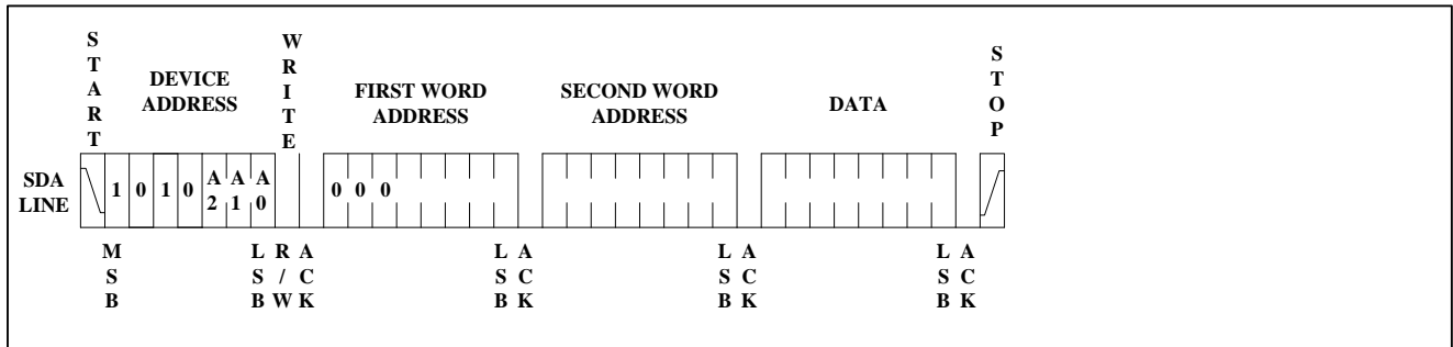
Figure 7. Byte Write
