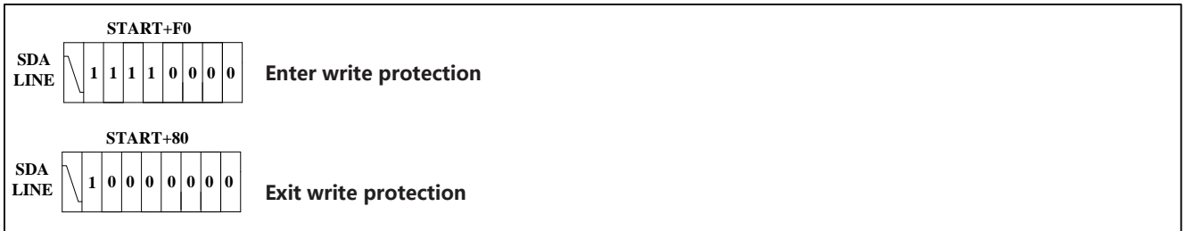
Figure 9. Soft Write Protection
