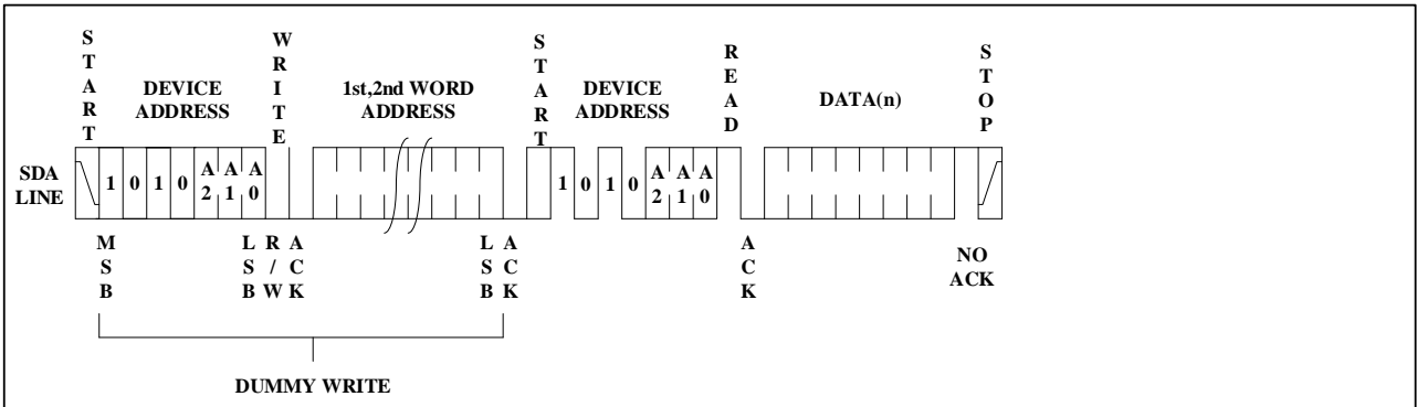
Figure 11. Random Read
