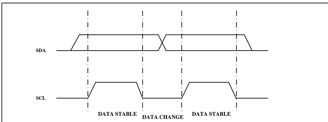
Figure 2. Data Validity
