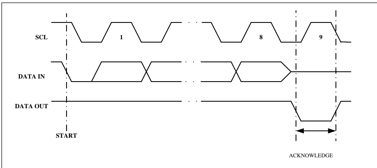
Figure 4. Output Acknowledge
