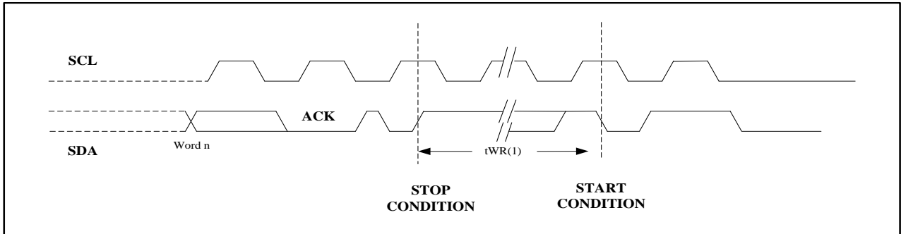
Figure 14. SCL: Serial Clock, SDA: Serial Data I/O
