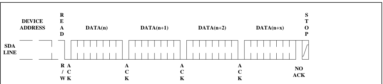
Figure 12. Sequential Read
