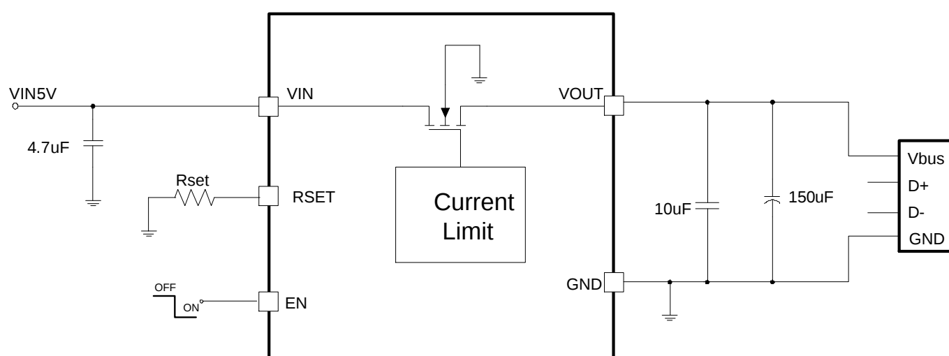
Figure 1. Typical application
