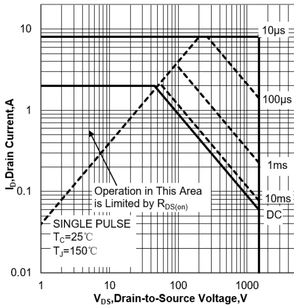
Figure 1a Safe Operating Area (No FullPAK)
