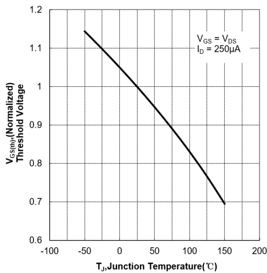
Figure 8 Typical Theshold Voltage vs Junction Temperature
