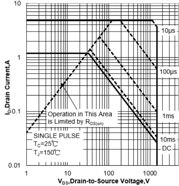
Figure 1b Safe Operating Area (FullPAK)
