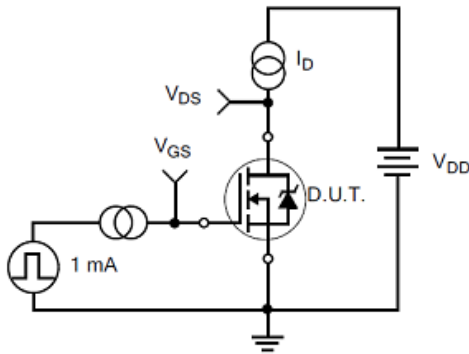
Figure 12 Gate Charge Test Circuit
