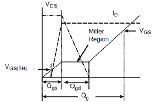
Figure 13 Gate Charge Waveforms
