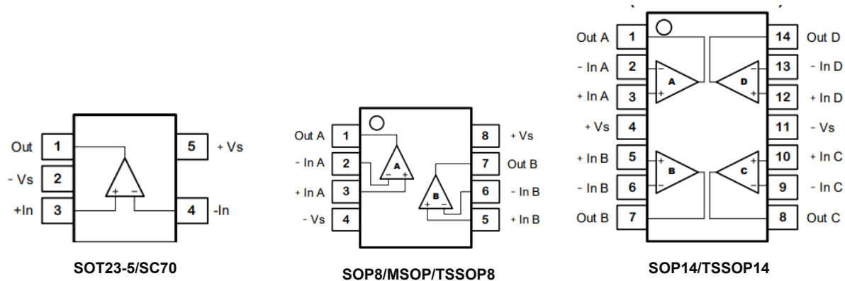
Figure 1. Pin Assignment Diagram
