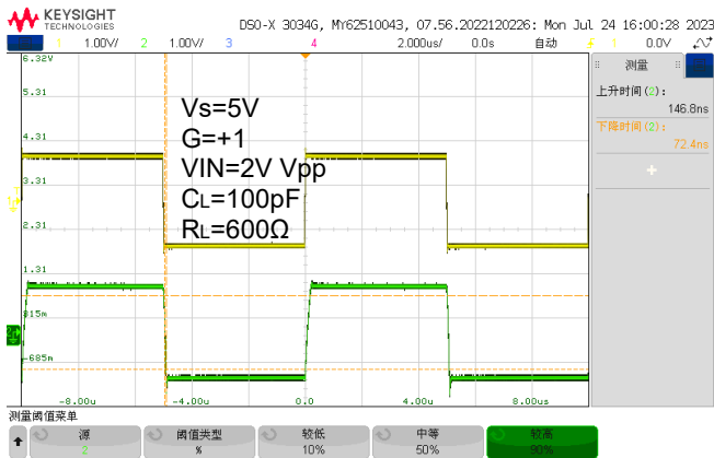
Slew Rate
