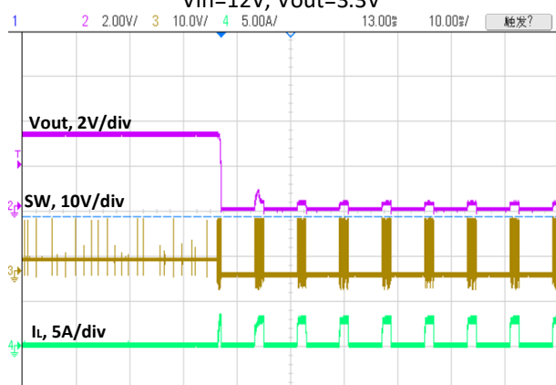
Short Circuit Wave
