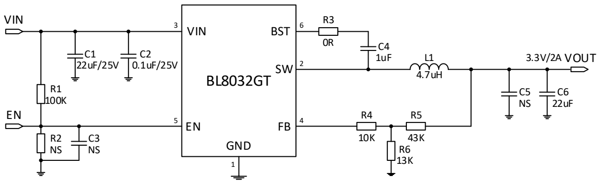
Figure 4. 12V VIN, 3.3V/2A
