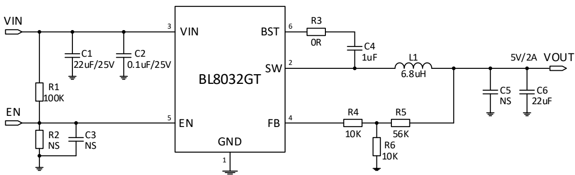
Figure 3. 12V VIN, 5V/2A
