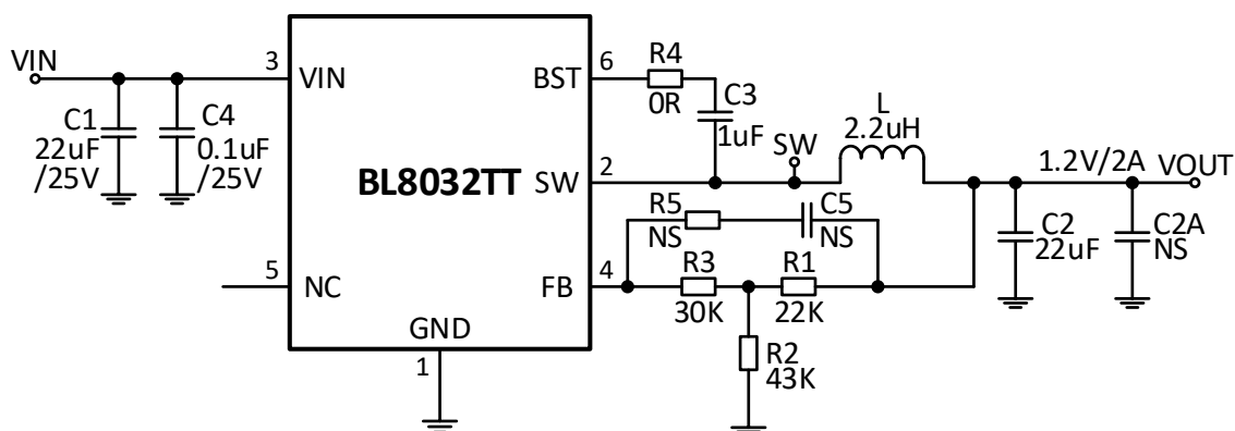
Figure 7. 12V VIN, 1.2V/2A
