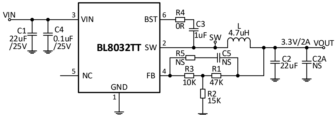
Figure 4. 12V V_{IN} , 3.3V/2A
