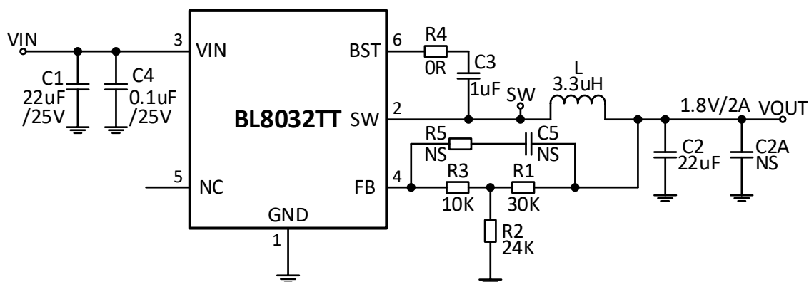
Figure 6. 12V VIN, 1.8V/2A
