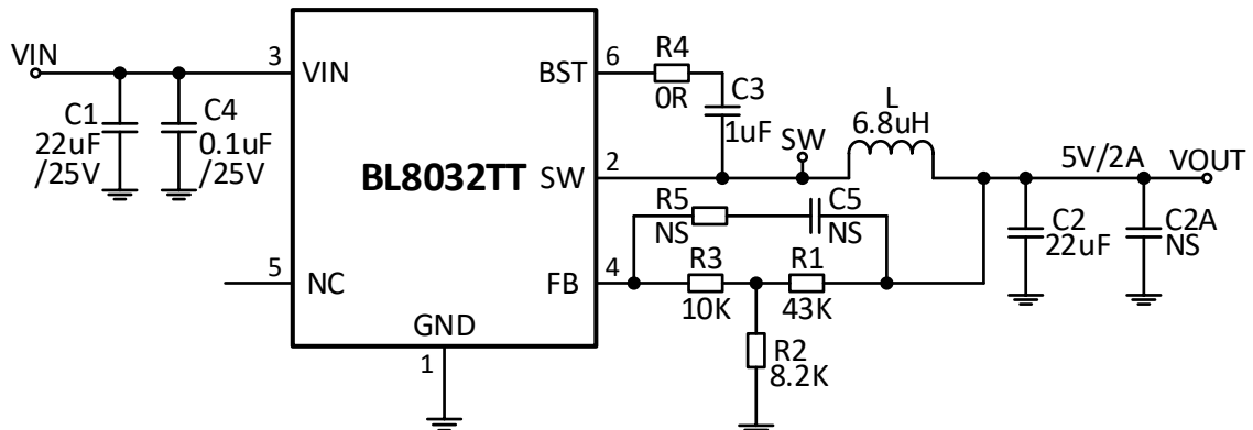
Figure 3. 12V V_{IN} , 5V/2A
