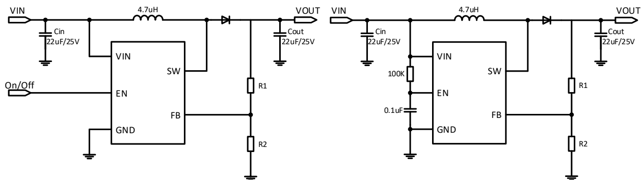
Figure 1. BL8042D typical application circuit
