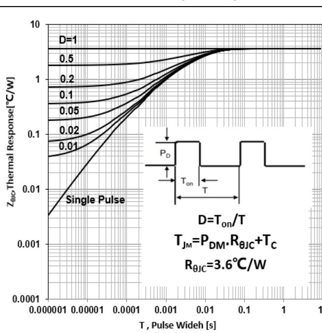
Figure 28. Diode Transient Thermal Impedance vs Pulse Width(TO220F)
