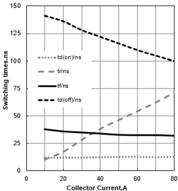
Figure 19. Typical Switching Times vs Collector Current ( T_J=25^\circ C , V_{CE}=400V , V_{GE}=15/0V )
