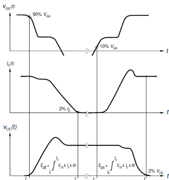
Figure 3. Definition of switching losses
