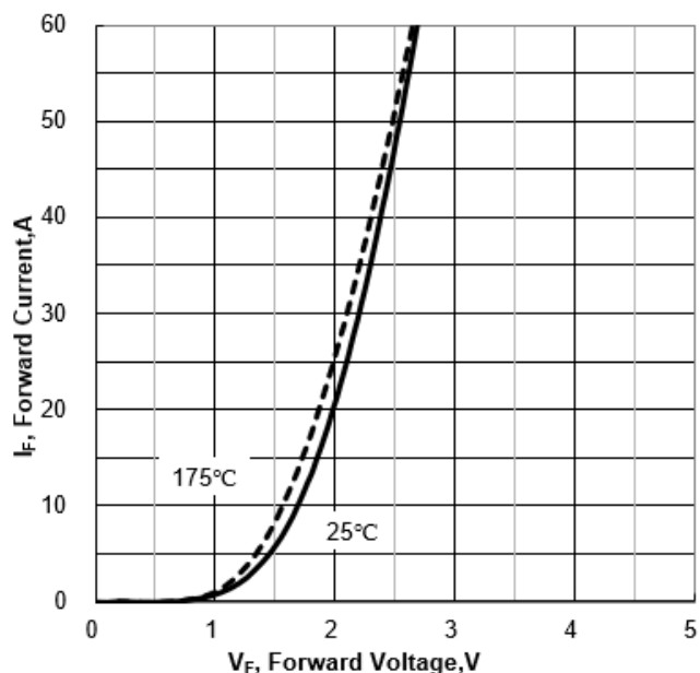
Figure 14. Typical Diode Forward Current vs Forward Voltage
