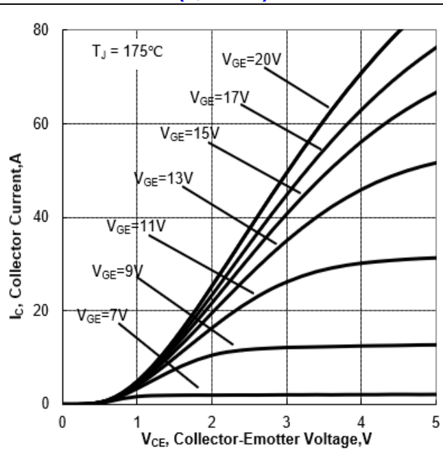
Figure 10. Typical Output Characteristics ( T_J=175^\circ\text{C} )
