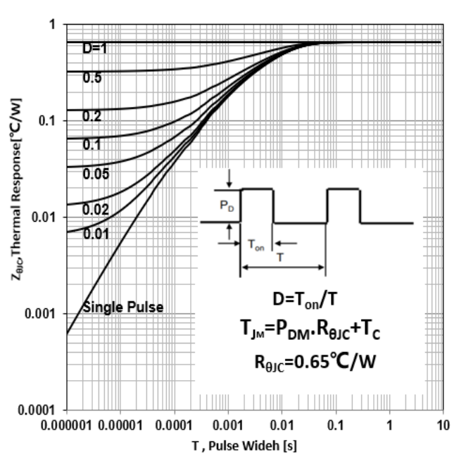
Figure 30. Diode Transient Thermal Impedance vs Pulse Width(TO247)
