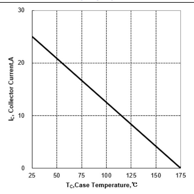
Figure 8. Collector Current vs Case Temperature for TO220F
