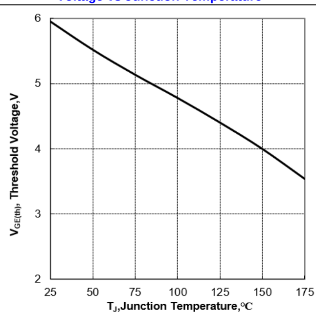
Figure 12. Typical Gate-Emitter Threshold Voltage vs Junction Temperature
