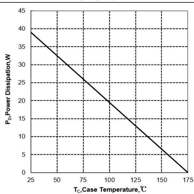
Figure 6. Power Dissipation vs Case Temperature for TO220F
