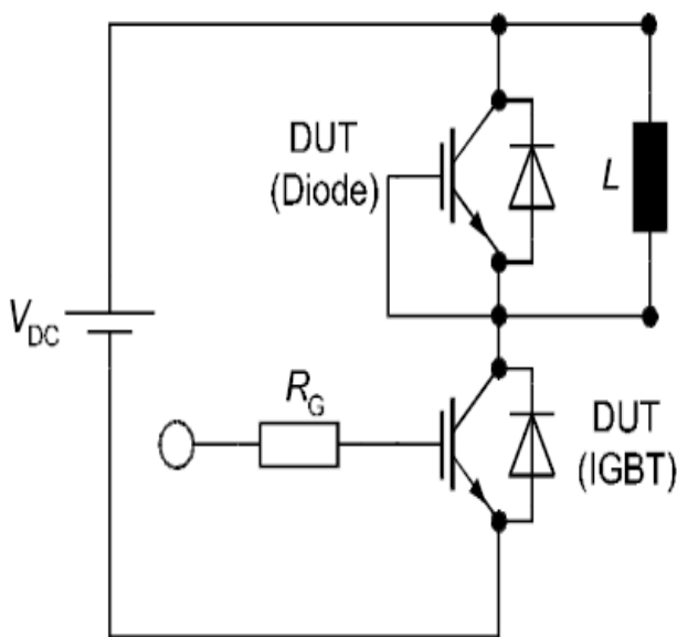
Figure 1. Inductive Switching Test Circuit
