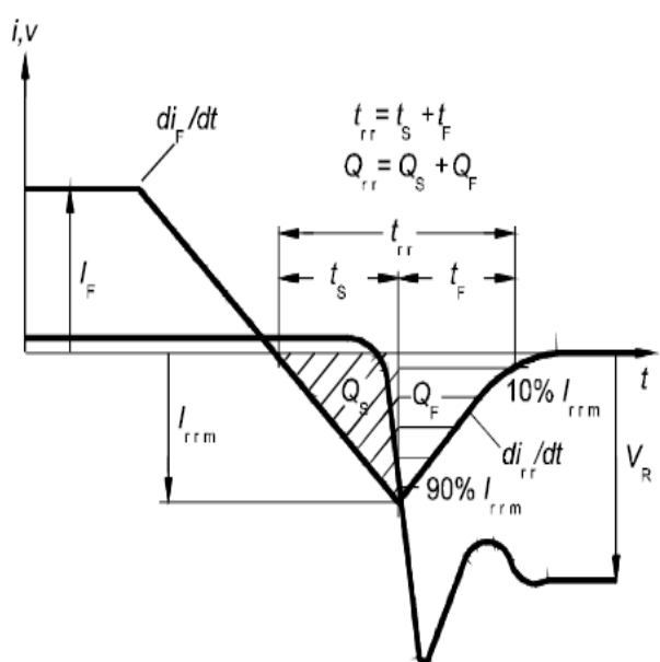
Figure 4. Definition of diode switching characteristics
