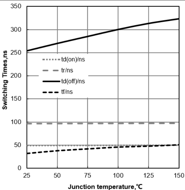
Figure 11. Typical Switching Times vs Junction Temperature ( V_{CE}=600\text{V} , V_{GE}=15/0\text{V} , I_C=40\text{A} )
