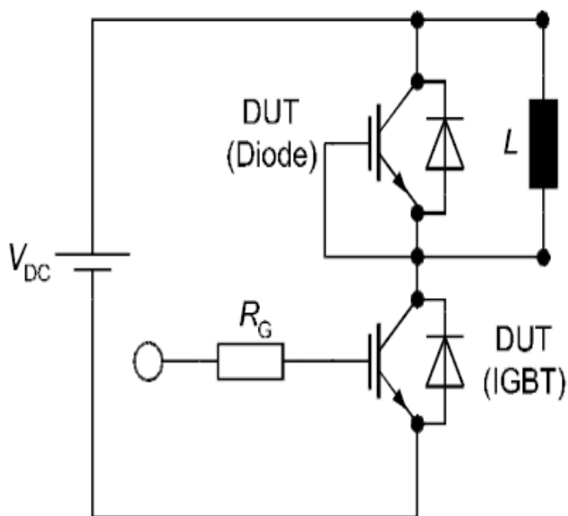
Figure 1. Inductive Switching Test Circuit
