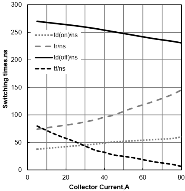
Figure 13. Typical Switching Times vs Collector Current ( T_J=25^\circ\text{C} , V_{CE}=600\text{V} , V_{GE}=15/0\text{V} )
