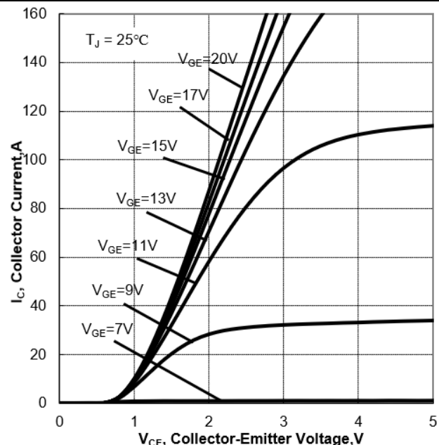
Figure 7. Typical Output Characteristics ( T_J=25^{\circ}C )
