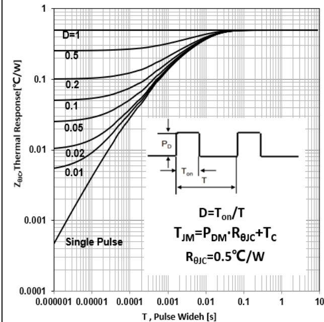
Figure 23. IGBT Transient Thermal Impedance vs Pulse Width(TO3PN/TO247)
