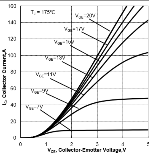
Figure 8. Typical Output Characteristics ( T_J=175^{\circ}C )
