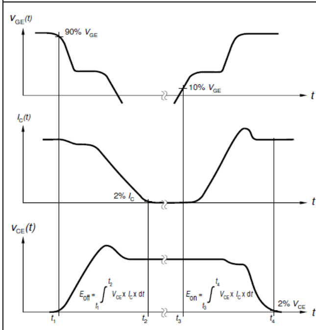
Figure 3. Definition of switching losses
