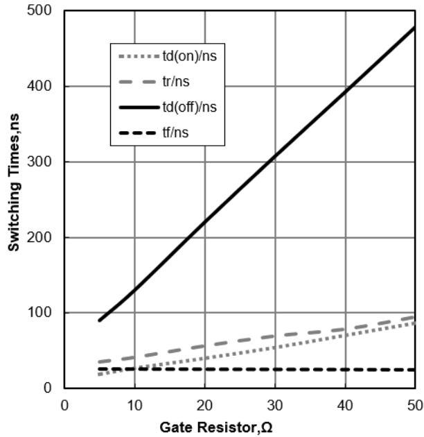
Figure 13. Typical Switching Times vs Gate Resistor ( T_J=25^\circ\text{C} , V_{CE}=400\text{V} , V_{GE}=15/0\text{V} , I_C=40\text{A} )
