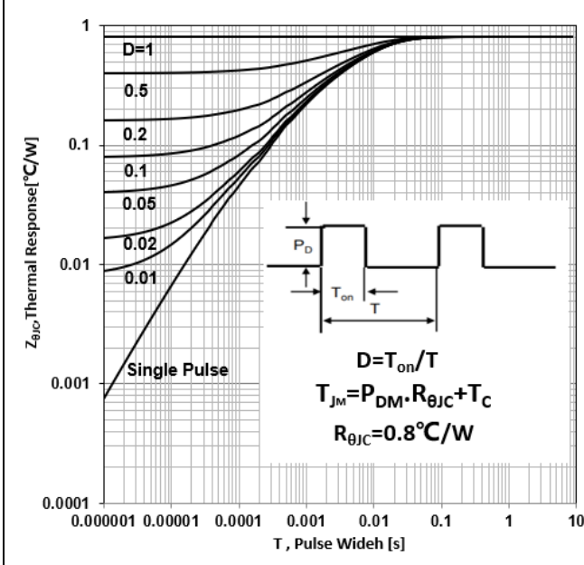
Figure 25. Diode Transient Thermal Impedance vs Pulse Width(TO247/TO3PN)
