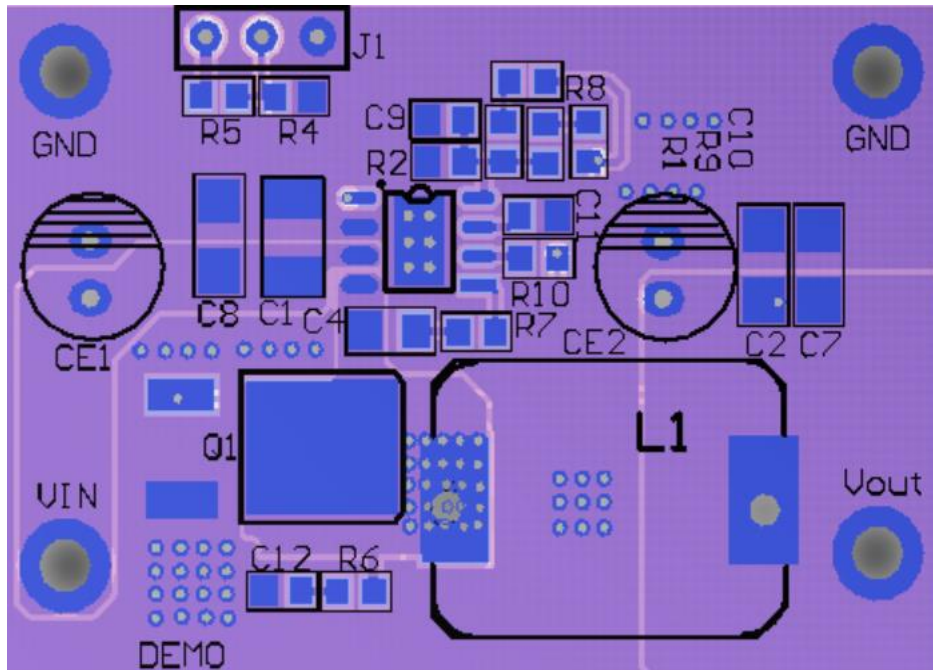
Top Layout
