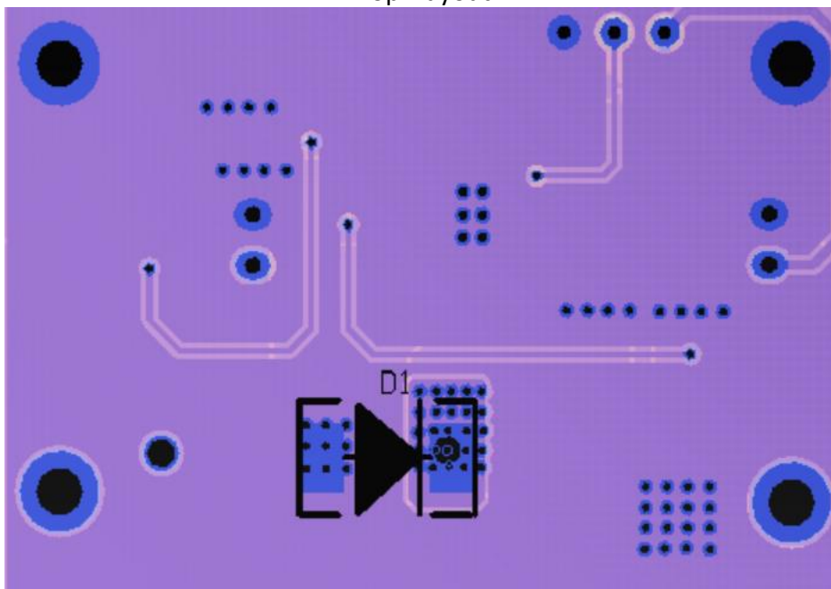
Bottom Layout
