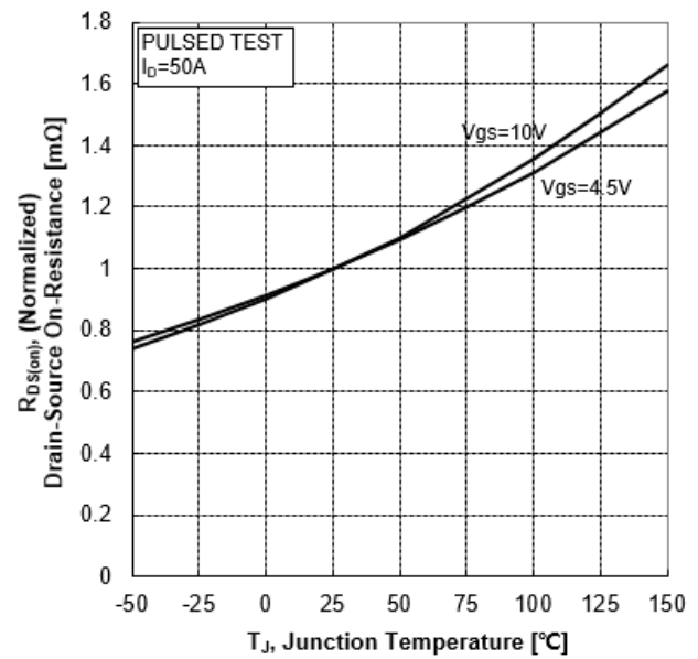
Figure 9. Normalized On-Resistance vs Junction Temperature
