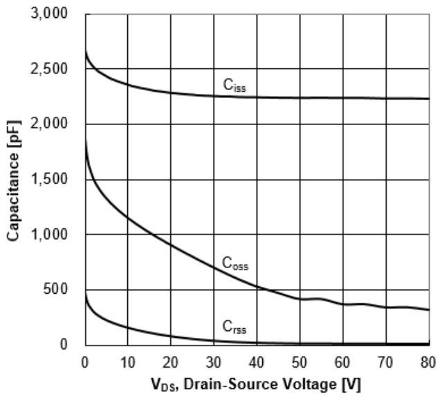
Figure 12. Capacitance Characteristics
