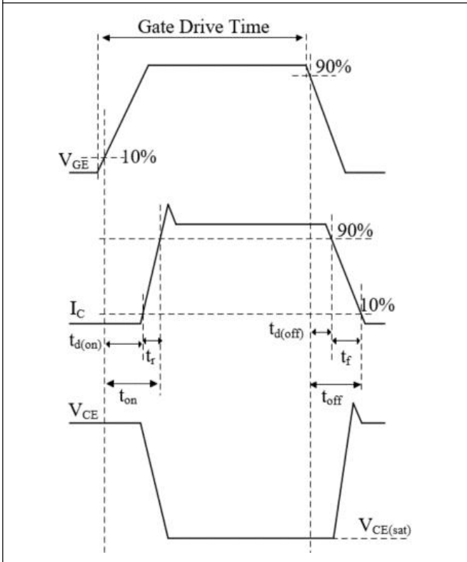
Figure 20 Switching Waveforms
