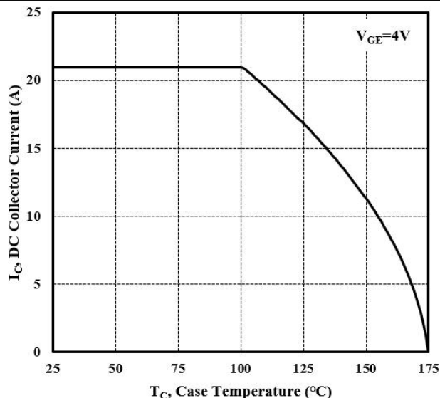
Figure 6. DC Collector Current vs Case Temperature
