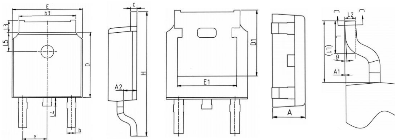
TO-252 Package
